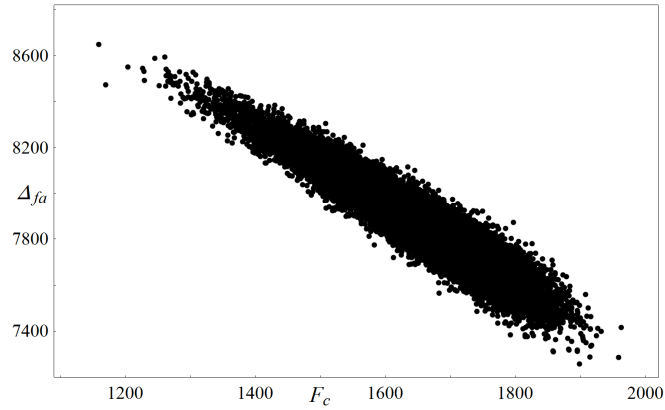
Fig. 11. Size of final catastrophic avalanche \Delta_{fa} vs. total critical force F_c in 2D system for LLS rule. Figure is based on 30 000 samples, each containing N = 10^4 pillars
