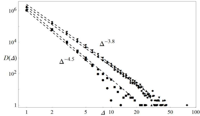
Fig. 9. Avalanche size distributions in 2D system for LLS variants - load transfer to: one nearest neighbour (circles), two nearest neighbours (squares), three nearest neighbours (diamonds), four nearest neighbours (up triangle), five nearest neighbours (down triangle). Simulation results are based on 1000 samples, each containing N = 10^4 pillars
