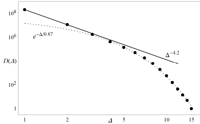
Fig. 10. Avalanche size distribution in 1D system for LLS with load transfer to one right neighbour. Figure is based on 200 000 samples, each containing N = 10^4 pillars
