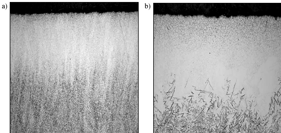
Fig. 2. The samples of microstructure of surface layer steel after carburizing, T = 1173 \text{ K} , etched in nital, magn. 50x, a) \tau = 3 \text{ h} , b) \tau = 12 \text{ h} [9]
