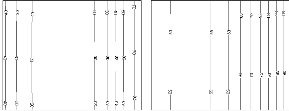
Fig. 1. Temperature distribution for times 10 and 50 second - 1 example (plane x_2 = 0.0225 m)
