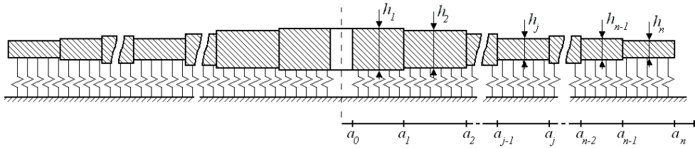
Fig. 1. A stepped annular plate resting on Winkler elastic foundation
