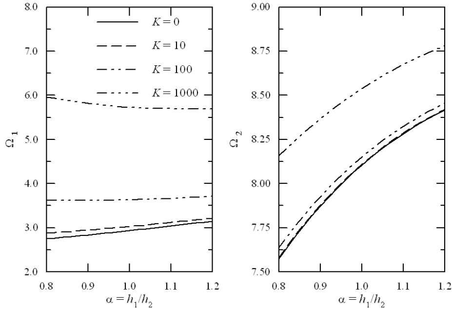
Fig. 2. Values of non-dimensional frequency parameter \Omega_{2,i} = \sqrt[4]{\rho h_2 \omega^2 a^4 / D_2} ( i = 1, 2 ) as a function of parameter \alpha = h_1/h_2 ; b/a = 0.4 , c/a = 0.7 , \nu = 0.3
