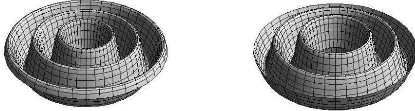
Fig. 2. The Green's functions for exterior Helmholtz problems (a) with the Dirichlet boundary condition, (b) with the Neumann boundary condition, n = 0 , \Omega = 2
